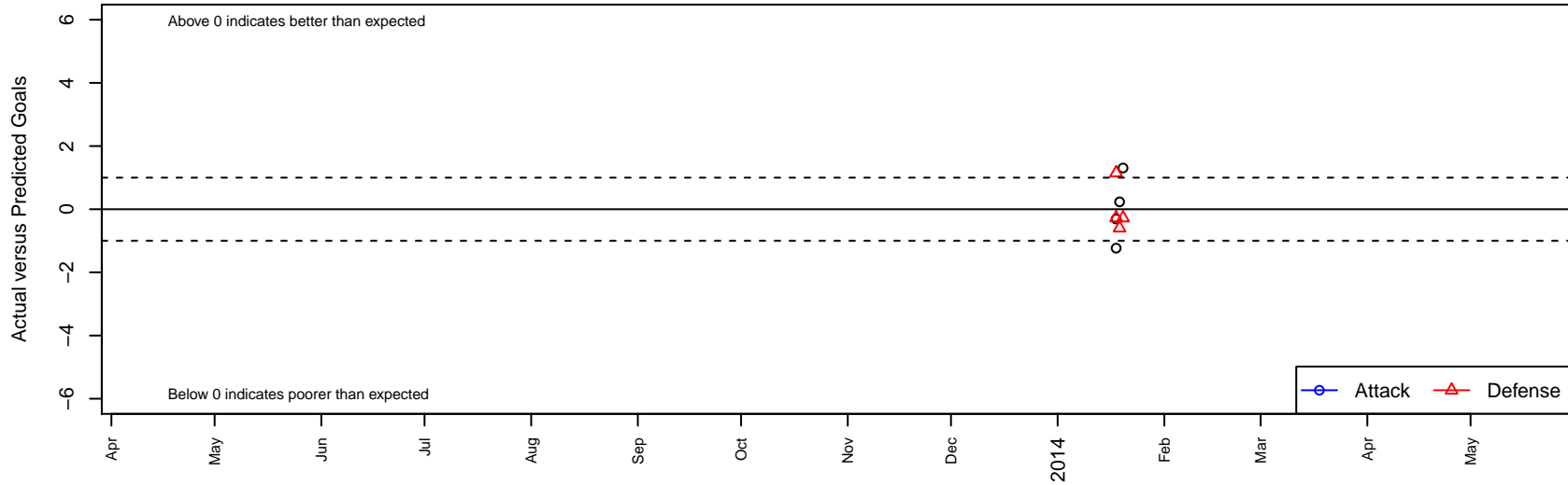
Montana United B95 Dots are actual minus expected GF (blue circles) and GA (red triangles). Blue line is smoothed change in attack strength. Red is smoothed change in defense strength.
